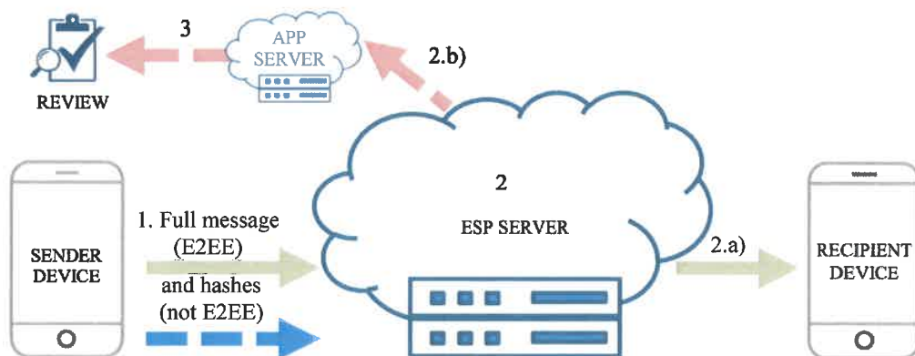
Figure 5: on-device hashing with matching at server
