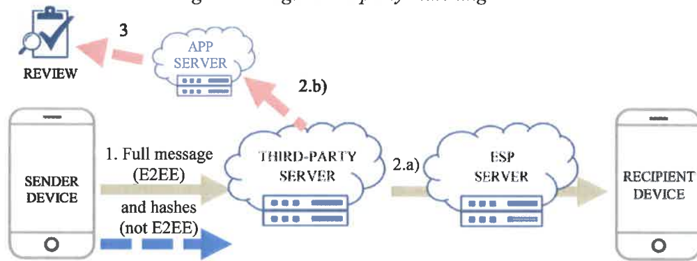
Figure 9: single third-party matching
