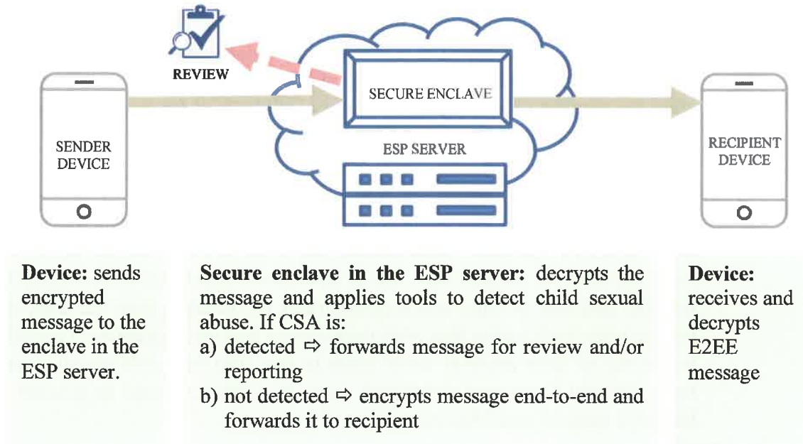
Figure 8: secure enclaves in the ESP server
